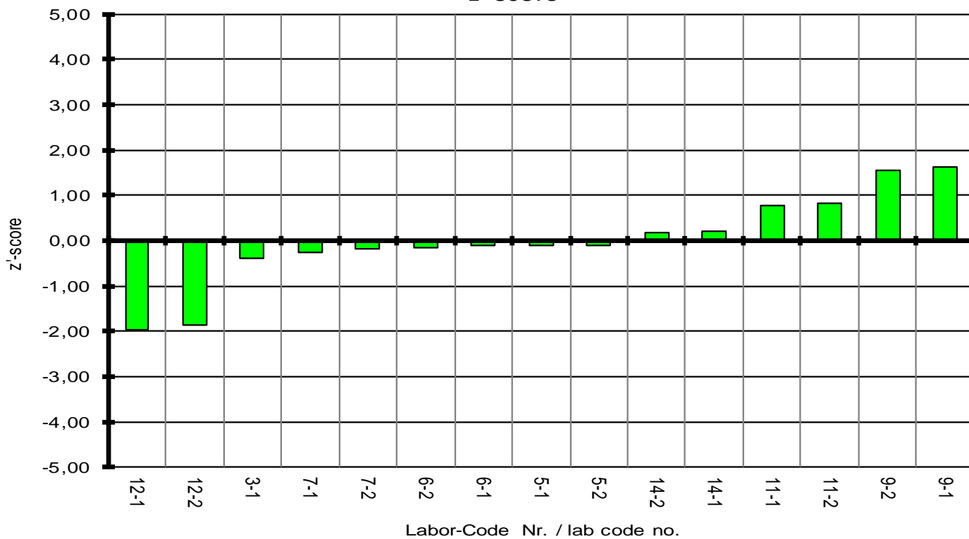
z'-score
